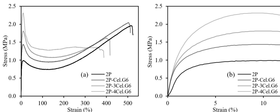
Figure 7. Stress x strain graph for (a) Parafilm® films and composite films containing one, three or four cellulose sheets of 6 m/g 2 (average curve); (b) enlargement of a.
